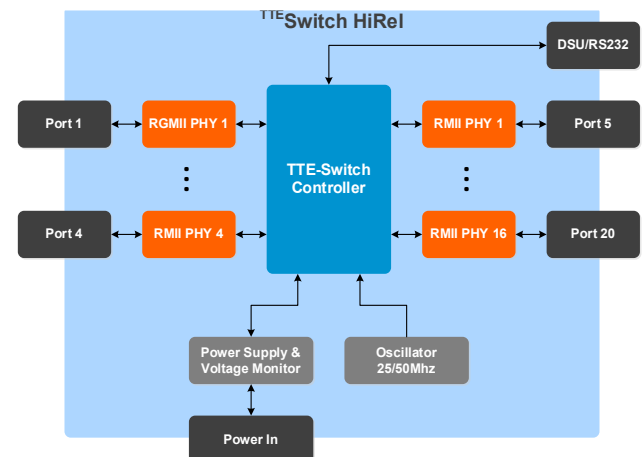
Block diagram of components in TTESwitch Mythos
